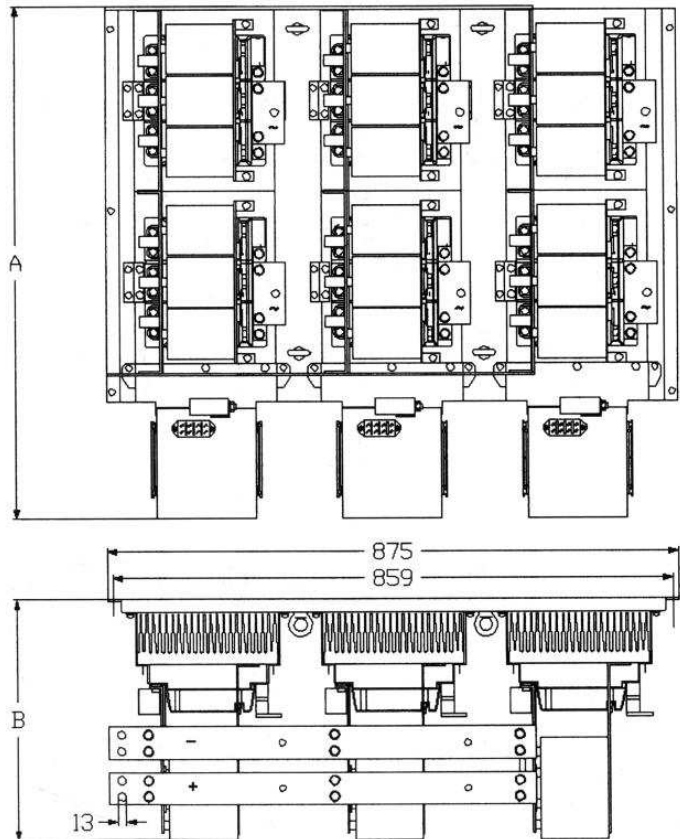
2. Application example using SKiPs and heatsink P 16 to give an IGBT inverter
