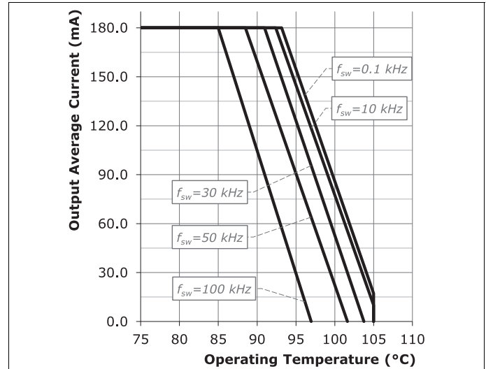
Fig. 2: Output Average Current
