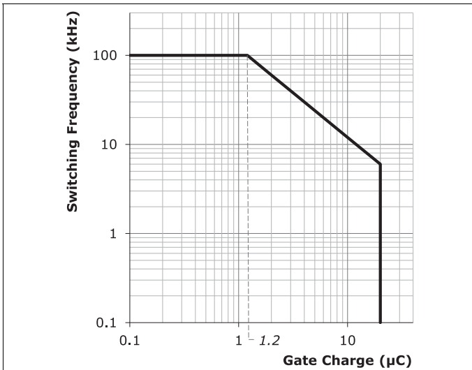
Fig. 1: Maximum Switching Frequency
